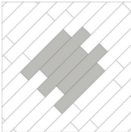
LAYING TILES WITH DISTANCE 4/5, Laying Crooked
